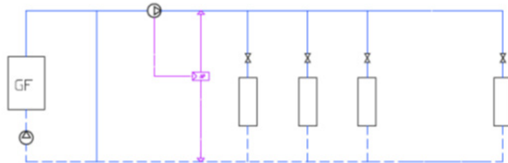
Scheme 1-a: double ring system with single chiller.
