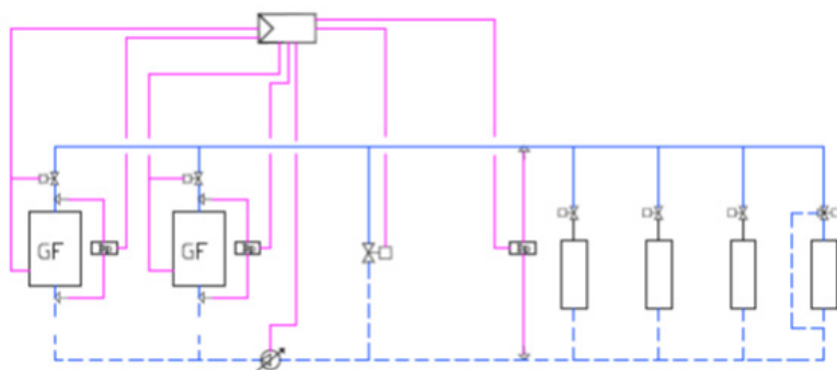
Diagram 2-b: variable flow single-ring system with more refrigeratori.
