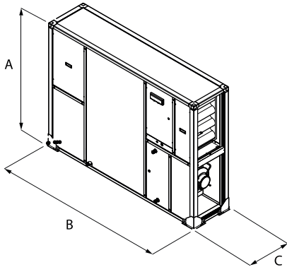
RPF 008 - 042 Installation vertical
