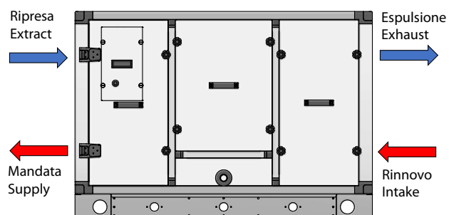
ERSR Horizontal Configuration Right delivery (top view)
