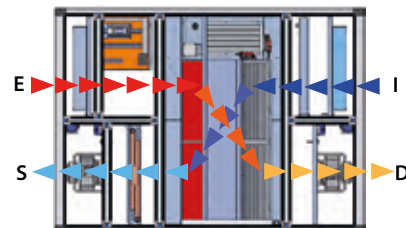
RPF Z Vertical Configuration Left delivery (view from accessible side)
